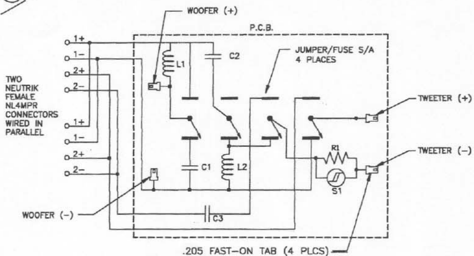
WIRING DIAGRAM
